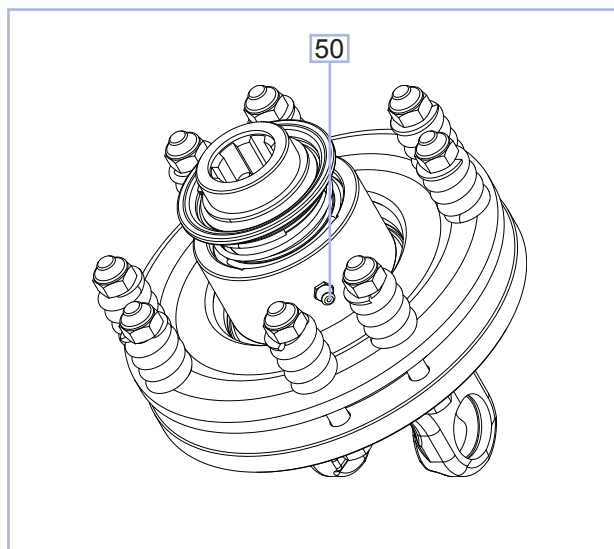
Friction overrunning clutch:
