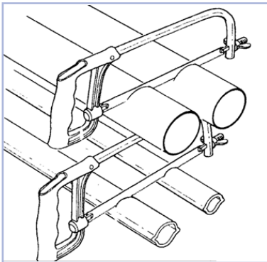
Figure J: Shorten
