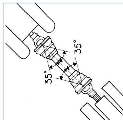
Figure G: Equal joint angles
