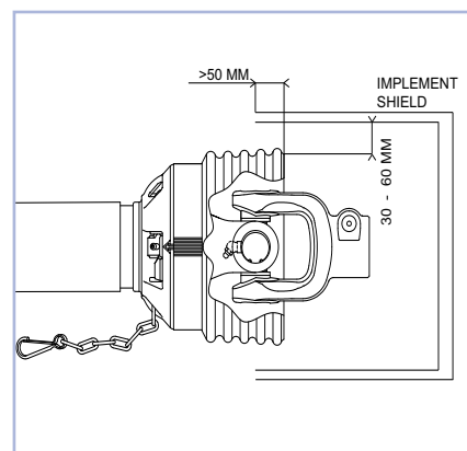
Figure F: Overlap
