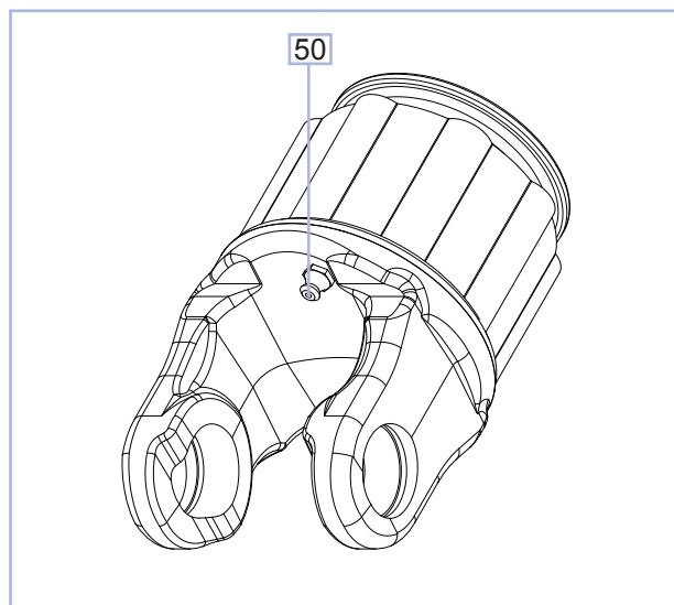
Ratchet clutch:
